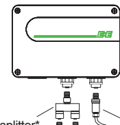
Y splitter* Lumberg RSC 5/7 RS485 network Lumberg RKC 5/7 power supply+ analogue output
